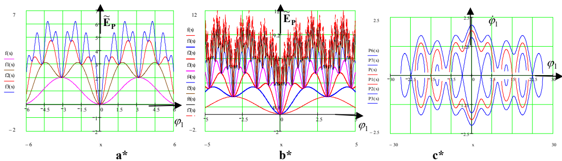
Figure 2. Multistep-coupled heavy rotors free nonlinear dynamics visualizations (Multipliers). a* and b* Potential energy curves families. c* Phase homoclinic trajectories potraits (constante energy curves). Homoclinic orbits layering for conservative system.
