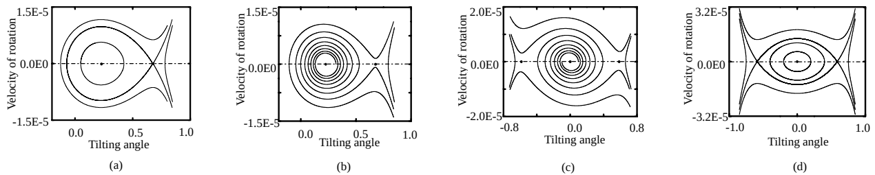
Fig.2 The phase portraits of the torsional RF MEMS switch with vdW torsion: (a) with voltage and without damping; (b) with voltage and damping; (c) without voltage and with damping; (d) without voltage and damping.
