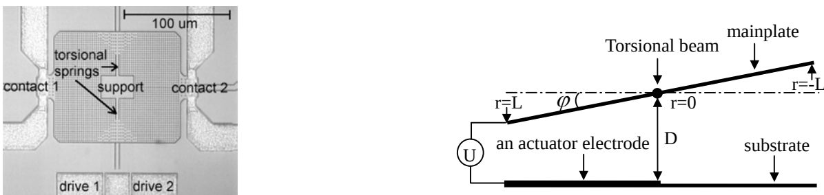
Fig.1. Topview micrograph and the schematic side view of the MEMS RF Switch
