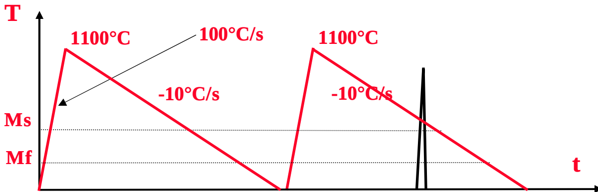
Figure 1: Free dilatometric test followed by predeformation test with a loading-unloading cycle applied before the starting of the martensitic transformation ( M_s ). The applied stress largely exceeds the yield limit of the austenitic phase.
