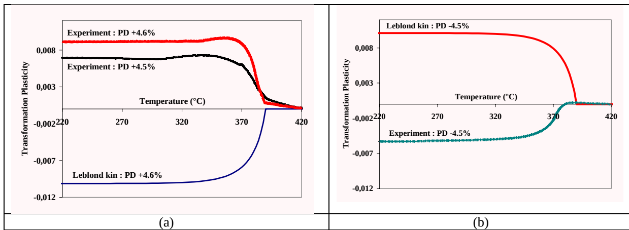
Figure 2: TRIP after pre-deformation (PD) test in which a loading-unloading cycle is applied before the starting of the martensitic transformation ( M_s ). The applied stress largely exceeds the yield limit of the austenitic phase. Comparison between experimental results and the predictions of Leblond's model: (a) Response after positive pre-deformation; (b) Response after negative pre-deformation.
