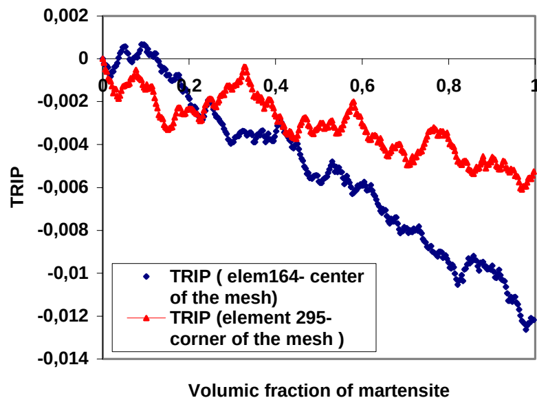
Figure 3: Numerical FE simulation of TRIP under constant applied stress. The result strongly depends on the choice of the first transformed element.
