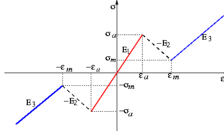
Figure 1: The three phase elastic material - equilibrium curve \sigma = \sigma_{eq}(\varepsilon) .
