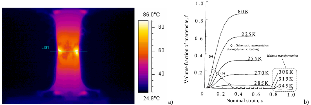
Fig.3. a – Temperature measurement during quasi-static tensile loading, \dot{\epsilon} = 10^{-2} \text{ s}^{-1} and t = 27.4 \text{ s} , b - Kinetics of phase transformation versus strain for different initial temperatures [2]
