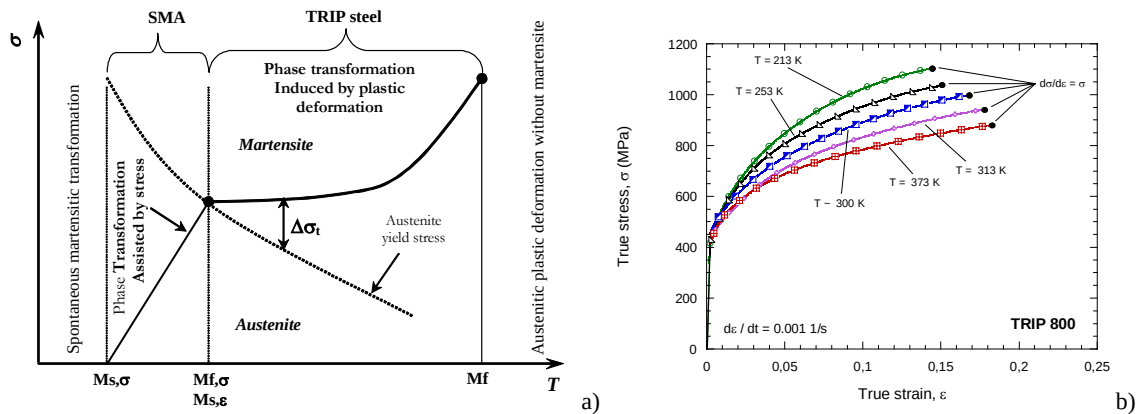
Fig.1. a - Schematic representation of the kinetic phase transformation with the initial temperature, b - Effect of the initial temperature on the plastic behavior in quasi-static tension
