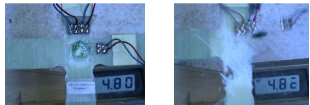
Figure 5: Failure of cruciform specimen geometry C at 48.2kN. Failure occurs in the biaxial loaded zone.
