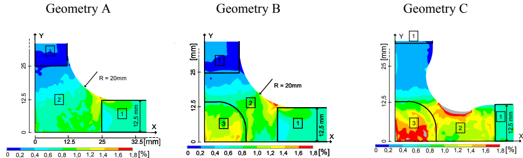
Figure 4: Finite element results for three cruciform geometries. First principal strains are shown.
