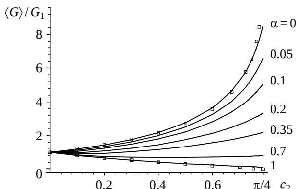
Fig. 1. Effective shear modulus \langle G \rangle ; G_2/G_1 = 20 .
