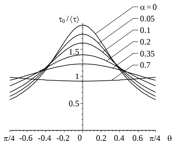
Fig. 2. Interfacial stresses \tau_0 ; G_2/G_1 = 20 , c_2 = 0.72 .
