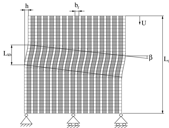
Figure 1: Specimen with 15 fibers showing the boundary conditions and the geometric imperfection.
