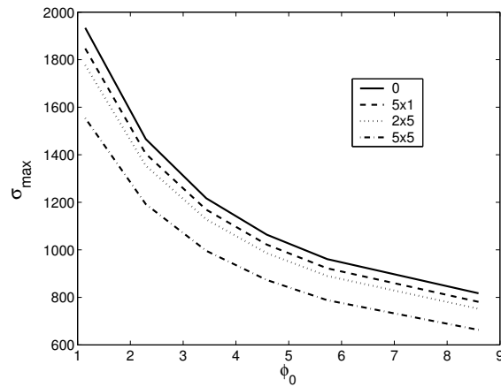
Figure 3: The compressive strength in MPa as a function of the initial fiber misalignment angle.
