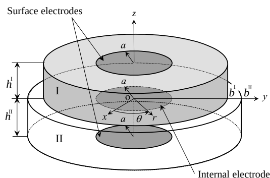
Fig. 1 Piezoelectric disk composite with circular electrodes
