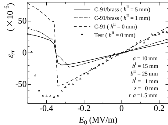
Fig.3 Radial strain \varepsilon_{rr} vs electric field E_0
