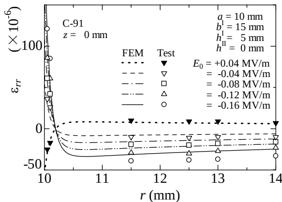
Fig.2 Radial strain \varepsilon_{rr} vs r : h^I=5 mm, h^{II}=0 mm
