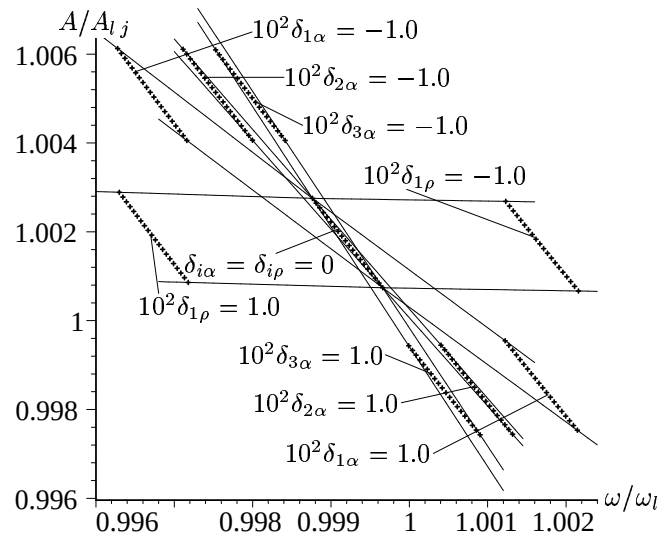
Figure 2. Nonlinear resonance as a function of the frequency and material properties ( j = 1 \dots 20 , i = 1, 2, 3 ).
