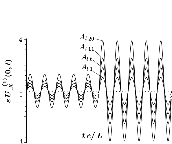
Figure 1. Variation of the boundary oscillation amplitude for the linear case ( n = 5 ).
