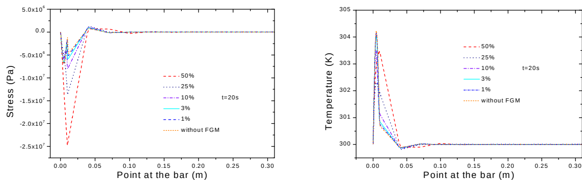
Figure2- Stress and temperature distributions in the domain of PSZ/steel FGM bar at the time 20s after submitted to temperature pulse 1000K with variation of material composition.
