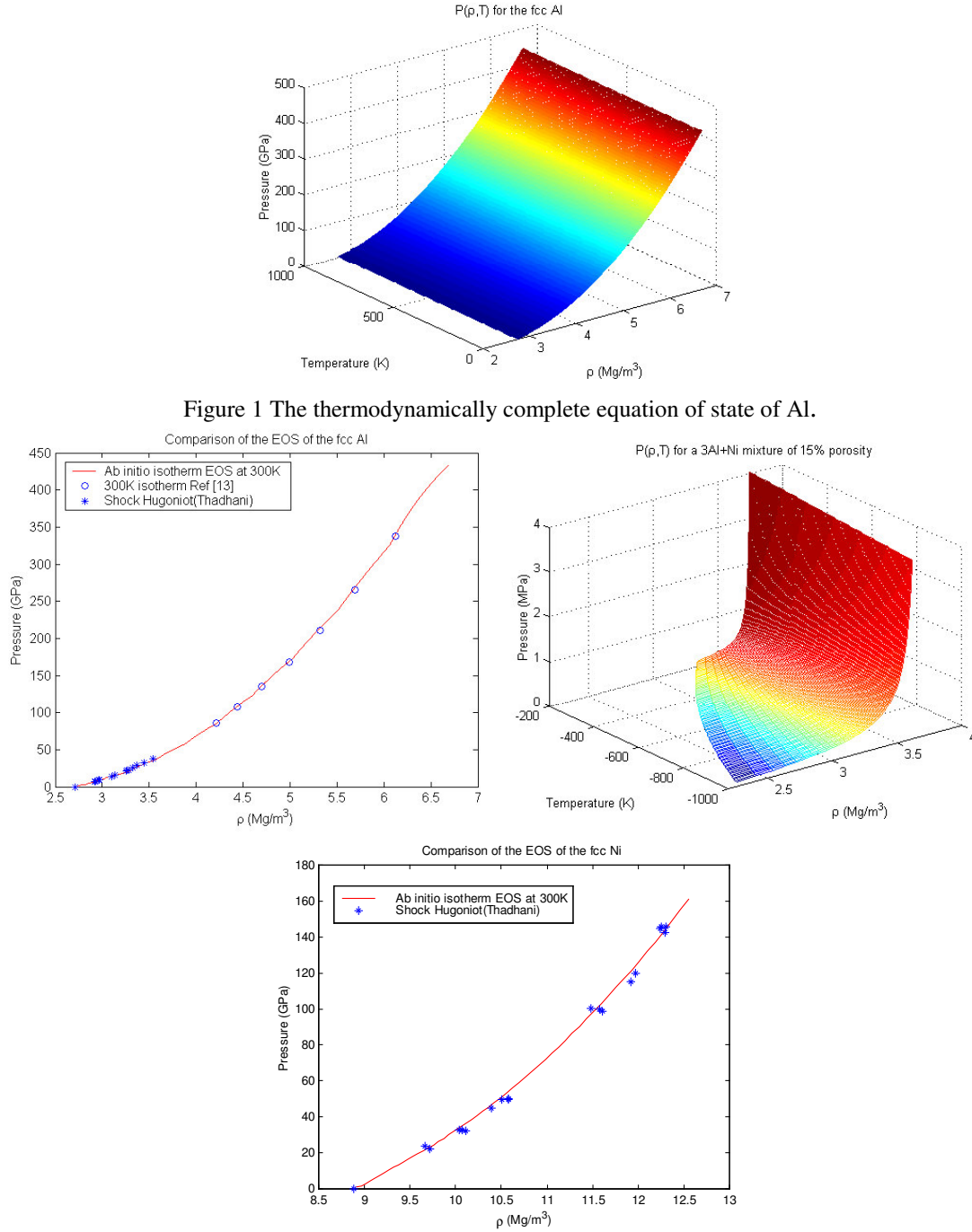
Fig.2-4: Comparison of EOS for Al & Ni with available Exptl. Data; EOS for the Mixture
