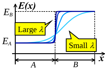
Fig.3 SIGMOID FUNCTION
