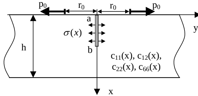
Fig.1 The schematic of the orthotropic functionally graded strip with an edge crack
