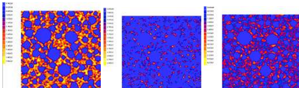
Figure 1. Simulation results for the damage calculus in a HSC under thermal loads (thermal strain fields, damage at 50°C, 120°C)
