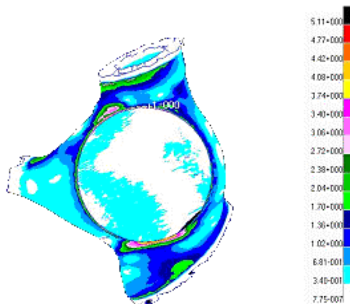
Fig. 4 The reduced stress distribution in cortical bone (scheme 5)
