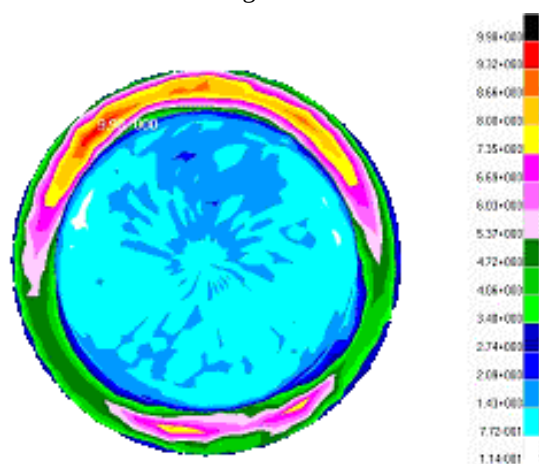
Fig. 5 The reduced stress distribution in artificial acetabulum (scheme 5)
