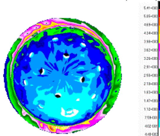
Fig. 6 The reduced stress distribution in cement layer (scheme 5)
