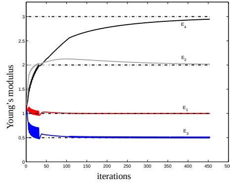
Figure 2. Young's modulus as a function of the iterations
