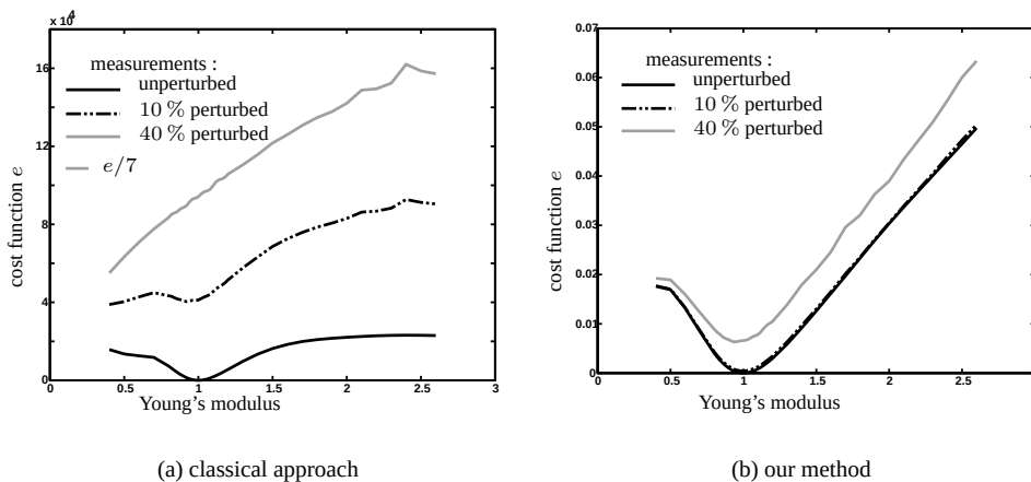
Figure 1. Variation of the error with E for different perturbation levels
