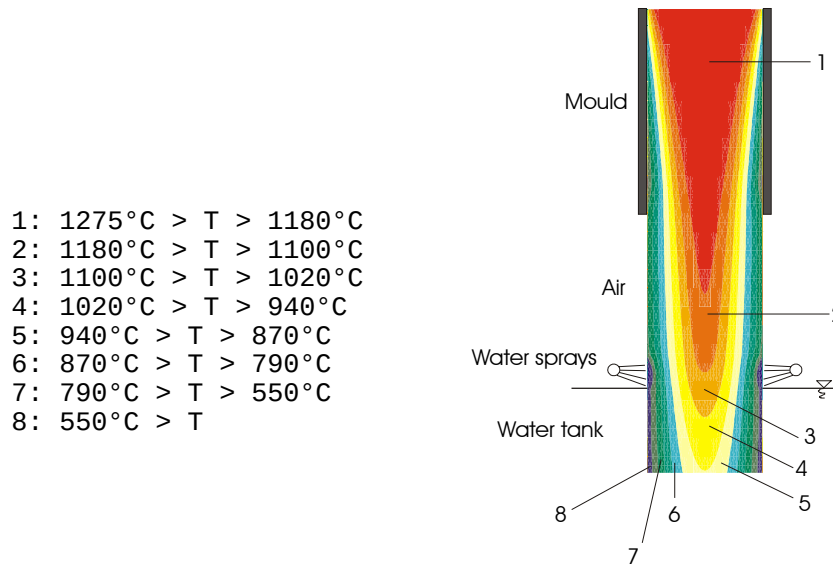
Figure 1 : Field temperature with the vertical slice model
