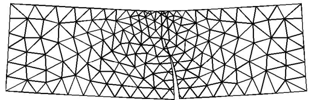
Figure 2: Propagation of excentered crack
