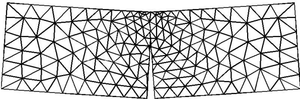
Figure 1: Propagation of centered crack
