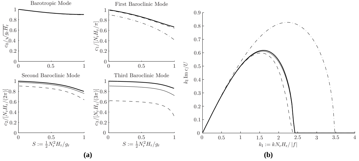
Figure 1. (a) Phase speed of long gravity waves as a function of the stratification in a reference state with no currents. (b) Growth rate of the most unstable Eady wave as a function of wavenumber. In both panels the exact result is indicated by a heavy-solid line, and the layered model predictions with dot-dashed (one layer), dashed (two layers), and light-solid (three layers) lines.
