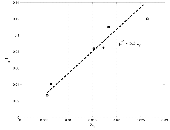
Figure 2: Mean distance between steps \mu^{-1} as a function of the Ozmidov length scale \lambda_0 , 2d results are with empty circles and 3d results with filled circles.
