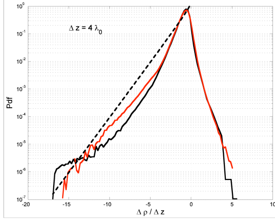
Figure 1: Pdfs of density gradient at vertical scale \Delta z = 4\lambda_0 for a wave of amplitude A = 0.256 , 3d results are represented in red and 2d results in black, theoretical prediction of the Hayes et al model with a dashed line.
