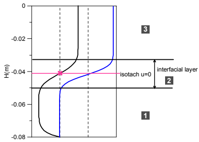
Figure 3. Velocity and density profiles
