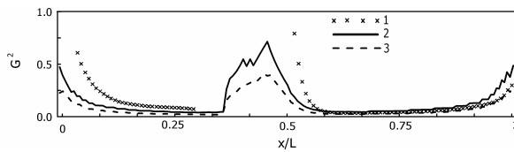
Figure 7. Composite Froude number along the strait calculated from the experiment 701 (1) vs. the computed one in the middle longitudinal section of the strait (2) and computed one using average flow parameters across the strait (3)
