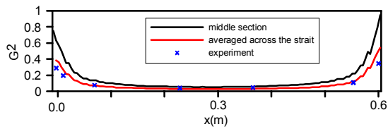
Figure 2. Composite Froude number
