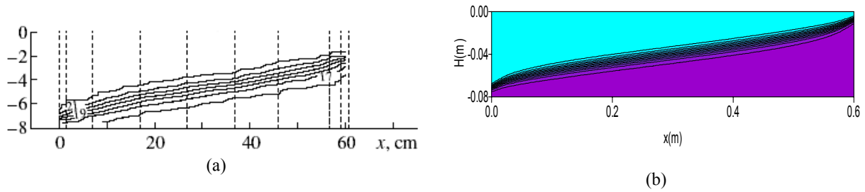
Figure 1. Temperature along the strait. (a) measured data, (b) computed results
