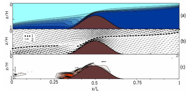
Figure 8. Computed density and velocity fields. (a) Contour plot of computed density from experiment 701. (b) Interface position in experiment 701 (1) and non-hydrostatic velocity field (2). (c) Absolute value of difference between hydrostatic and non-hydrostatic velocity fields.
