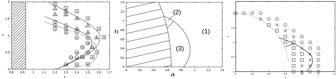
Fig. 1 FigMerger threshold of the Fig. 2 Three patterns found for a Fig. 3 Pattern map of nonlinear development of counter-rotating vortices with \alpha_{1,2}/\gamma_{1,2} = 0.3162 . \alpha_{1,2}/\gamma_{1,2} = 0.3162 .
