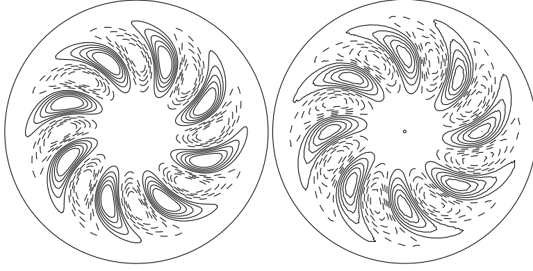
Figure 1. Contours of the radial flow in the equatorial plane. Left panel is the solution derived from the new theory and the solution on right panel is obtained from the fully three dimensional numerical simulations.
