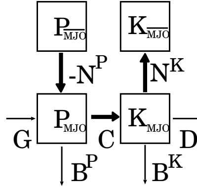
Figure 2: The schematics of the energy cycle identified for MJO in the LMDZ simulation.
