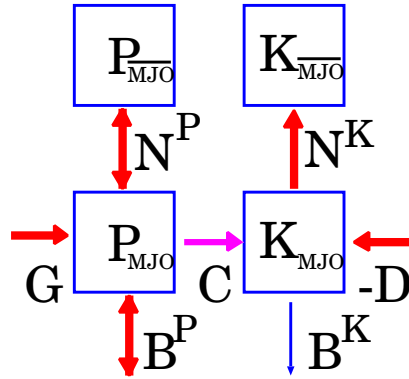
Figure 3: The schematics of the energy cycle identified for MJO in the
