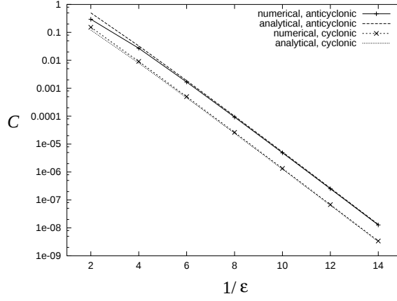
Figure 1. IGW amplitude C as a function of 1/\epsilon for sheared disturbances.
