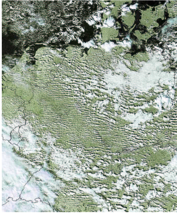
Figure 1: Clouds organized into rows due to roll-vortices in the atmospheric boundary layer.
