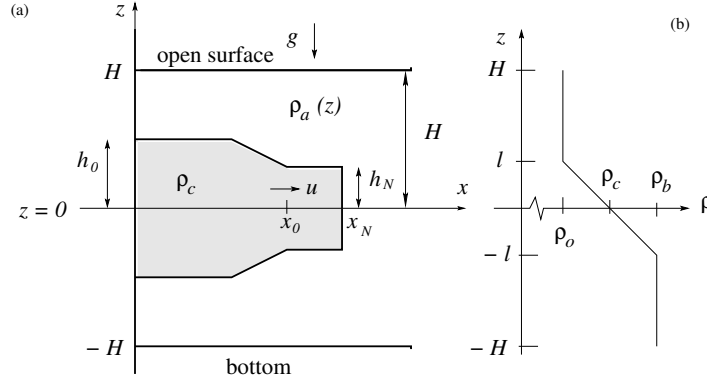
Figure 1: Schematic description of the system: (a) geometry after release from a rectangular lock; (b) density profile in the ambient (note \rho_c = 0.5(\rho_b + \rho_o) ). In dimensionless form, vertical and horizontal lengths are scaled with x_0 and h_0 , respectively. Velocity and time are scaled with U = (g' h_0)^{1/2} and x_0/U , where g' = (\rho_c/\rho_o - 1)g . The subscripts denote: N - nose (or front); a - ambient; b - bottom; c - current (intrusion); o - open surface.
