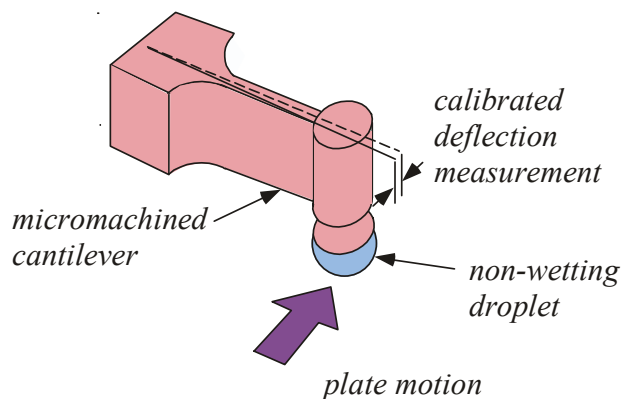
Figure 1. Schematic for non-wetting friction measurement.
