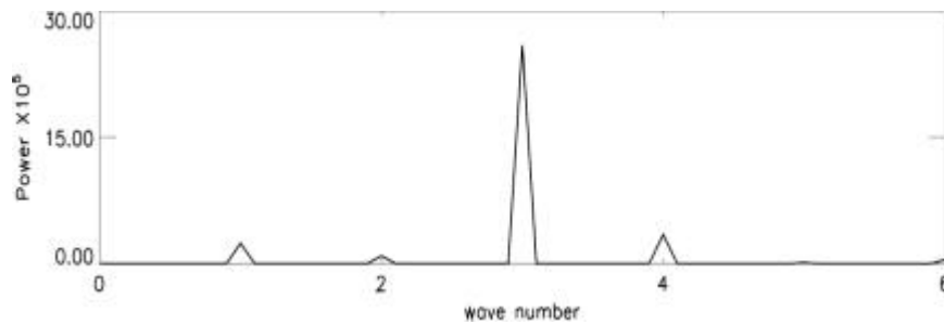
Fig.1. Spatial Fourier spectrum, Pr=4 , Ma=18000 .
