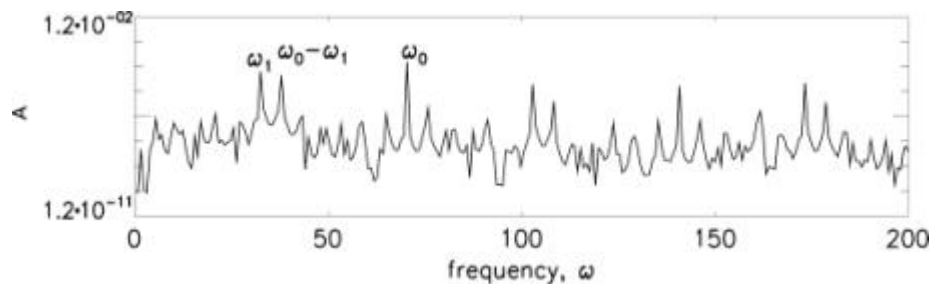
Fig.2. Temporal Fourier spectrum, Pr=4 , Ma=18000 .
