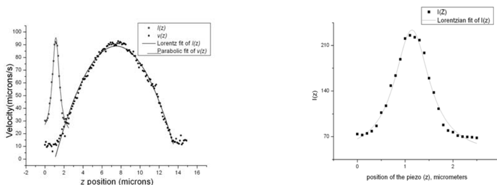
Figure 4 : a) velocity profile for glass
