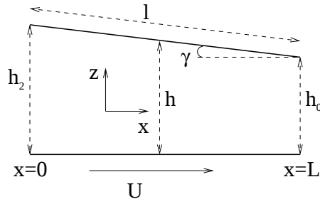
Figure 1: Geometry of a slider bearing.
