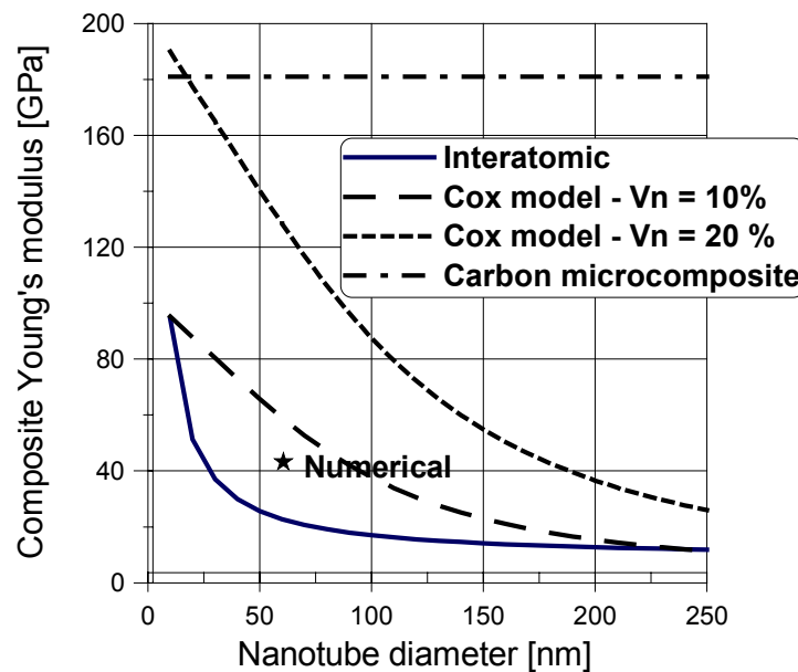
Fig.1 A comparison of mechanical properties for carbon micro- and nano- composites
