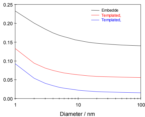
Figure 1: Size-dependent band structure shift due to surface energy effects
