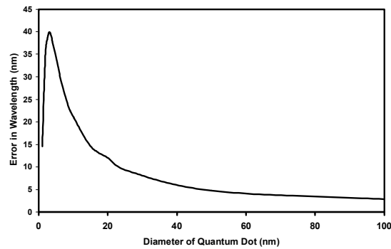
Figure 1: Size-dependent wavelength shift due to surface energy effects
