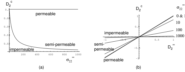
Figure 1. The crack face electric induction D_2^c for BSN with H_{24} = 0 .
