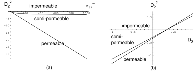
Figure 2. The crack face electric induction D_2^c for BSN with H_{24} \neq 0 .
