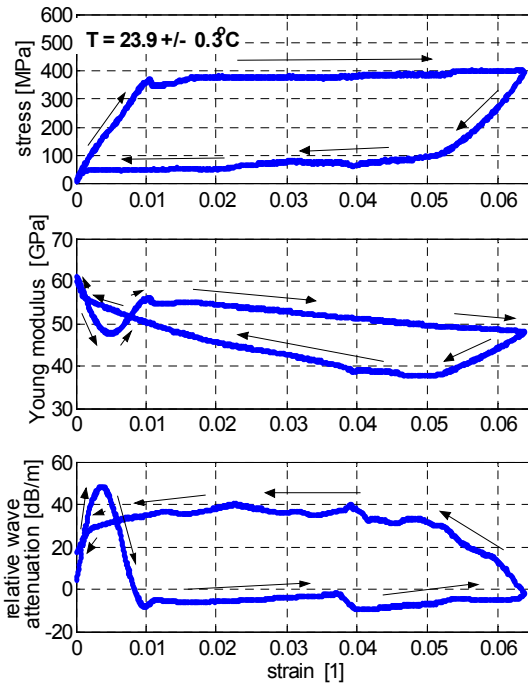
Figure 3: Stress and quantities, determined by ultrasound, during virgin loading of the tested NiTi wire.
