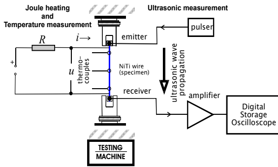
Figure1: Experimental arrangement
