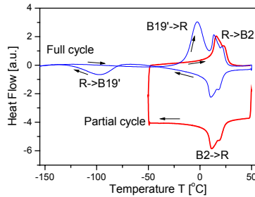
Figure 2: DSC record during full and partial cooling-heating cycles showing temperature ranges where individual transformation events take place.
