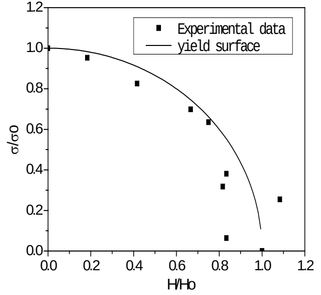
Figure 2. The dimensionless initial yield surface of Terfenol-D
