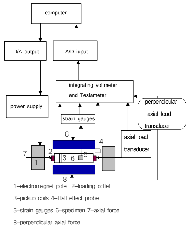
Figure 1: Schematic of the setup. The industrial PC controls the electromagnet supplier and monitors the magnetic H , magnetic induction B and the magnetostriction of specimens by an A/D-D/A interface card.
