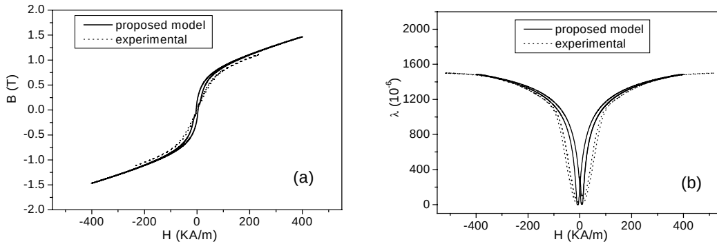
Figure 3. Comparison of the theoretical and measured results under magnetomechanical loading with 3MPa compressive stress: (a) the hysteresis curve; (b) the magnetostrictive curves.
