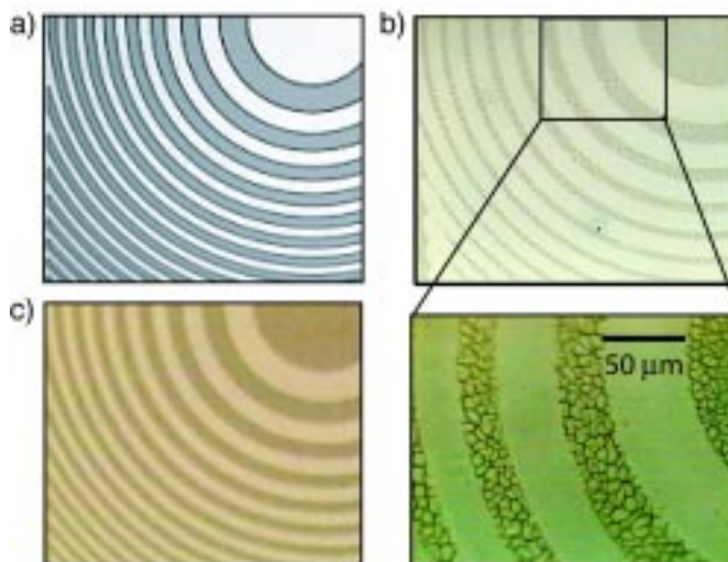
Fig. 1. Mediated deposition of PZT thin film: a) Master mold, b) selective cracking and decohesion over transferred SAM pattern, c) final patterned PZT film, light regions are PZT, dark regions are the Si substrate [1,2].
