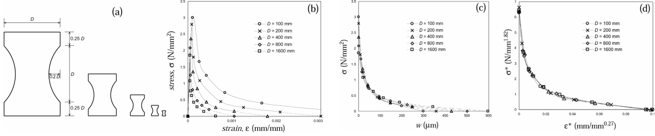
Figure 3: Tensile tests on dog-bone shaped specimens (a) by van Vliet [3]: stress-strain diagrams (b), cohesive law diagrams (c), fractal cohesive law diagrams (d). The dashed lines refer to extrapolated values.
