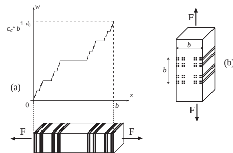
Figure 2: Fractal localization of the strain (a) and of the energy dissipation inside the damaged band (b).
