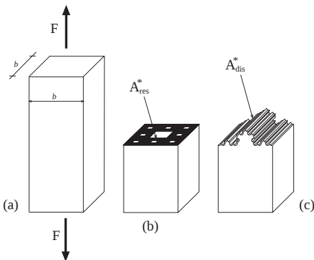
Figure 1: Tension specimen (a). Fractal localization of the stress upon the resistant cross section (b) and of the energy dissipation upon crack surface (c).
