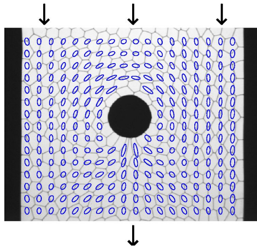
Figure 1. Analysed image from the experiment. The foam flows from top to bottom at a velocity of order 1 cm/s. The width of the channel is 10 cm and the typical size of bubbles is 5 mm. The ellipses represent bubble deformation, averaged over time at each point. With this representation one can visualise the deformation experienced by bubbles at the vicinity of the obstacle, compression uphill and stretching downhill [2] (picture M. Asipauskas).
