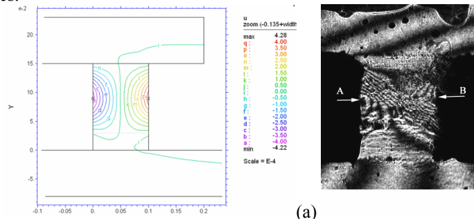
Figure 2 (a) Simulated horizontal displacement after 600 hours (b) U field fringe after 605 hours
