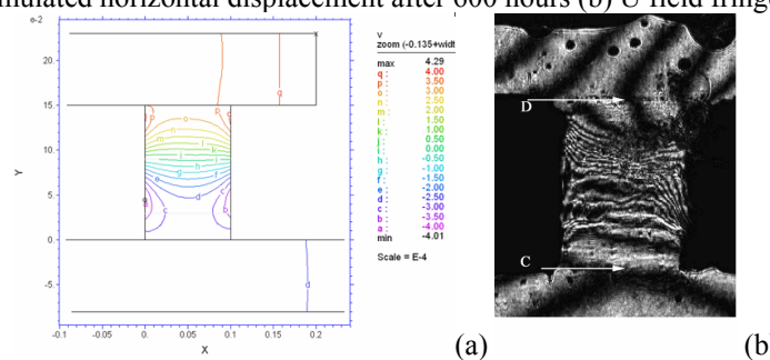
Figure 3 (a) Simulated vertical displacement after 600 hours (b) V field fringe after 605 hours
