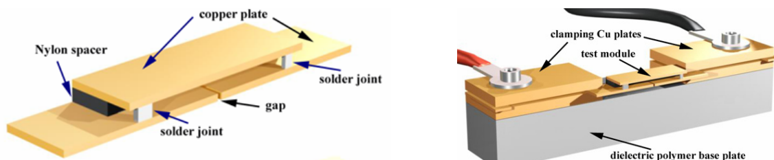
Figure 1 Scheme of the test module and the test fixture
