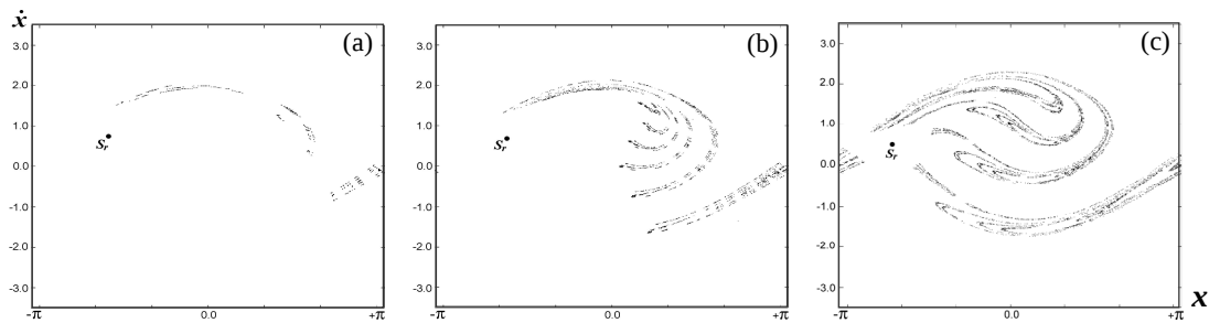
Fig. 1. Expansion of a chaotic saddle due to the Melnikov homoclinic bifurcation in a pendulum system (2), in the region of existence of a single attractor S_r ( \omega = 0.84 ); (a) F = 0.30 ; (b) F = 0.37 ; (c) F = 0.57 .
