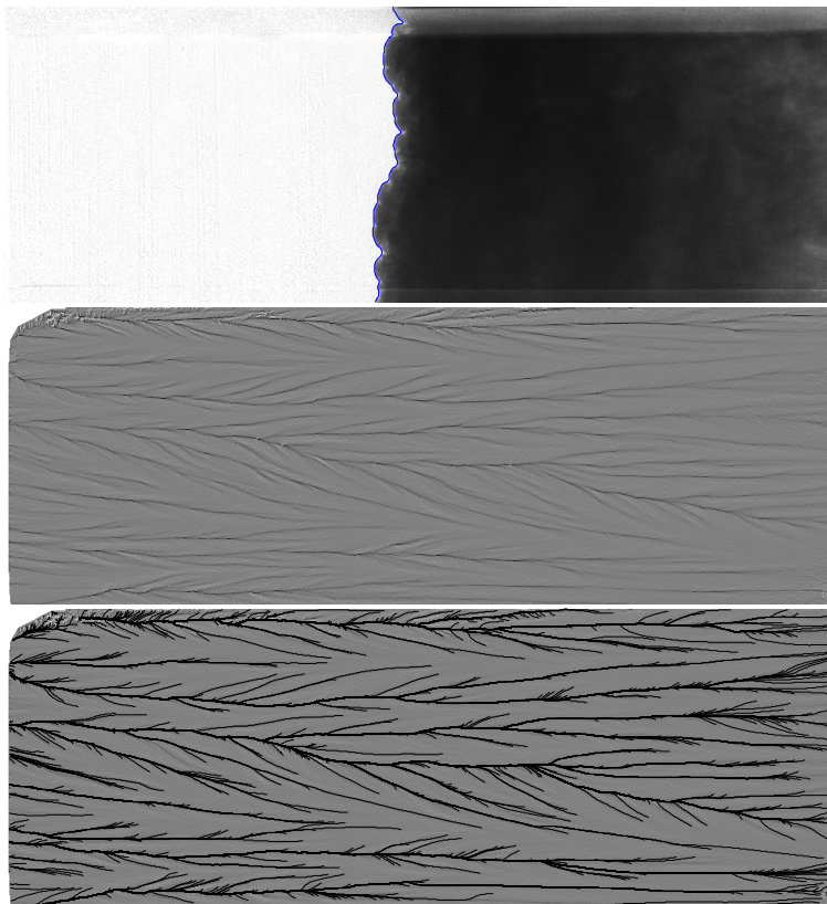
Figure 1. a) Contour mapping. The motion of the gravity current in all figures is right to left. b) Curvature of first arrival time field. Black corresponds to curvatures less than -2 (inverse pixels), white to great than +2, and the intensity is linear in between. c) Position of clefts superimposed on curvature picture
