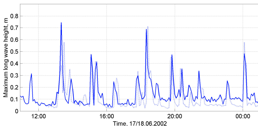
Fig. 1. The maximum height of the long-wave component (waves with periods exceeding 5 s and mostly representing wakes from high speed ships) near the western coast of the island of Aegna at the entrance of Tallinn Bay, at a distance of about 2 km from the ship lane on 17.06.2002 (solid line) and 18.06.2002 (dotted line). The significant height of the wind wave background is 40–60 cm on 17.06 and 30–40 cm on 18.06.
