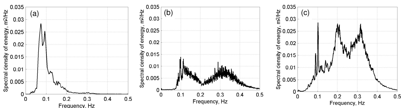
Figure 2. Daily mean joint energy spectra of wind waves and ship wakes in the coastal zone of Tallinn Bay at a distance of about 2 km from the ship lane (a) in perfectly calm conditions; (b) in the moderate wind conditions (the significant height of wind waves is about 40–60 cm, the temporal behaviour of the heights of long waves is given in Fig. 1, solid line); (c) in strong wind conditions (the significant height of wind waves is about 1 m and open sea swell with a period of about 5 s is also present). The measurement site for the panel (b) is located in the area where ships sail at moderate speeds.
