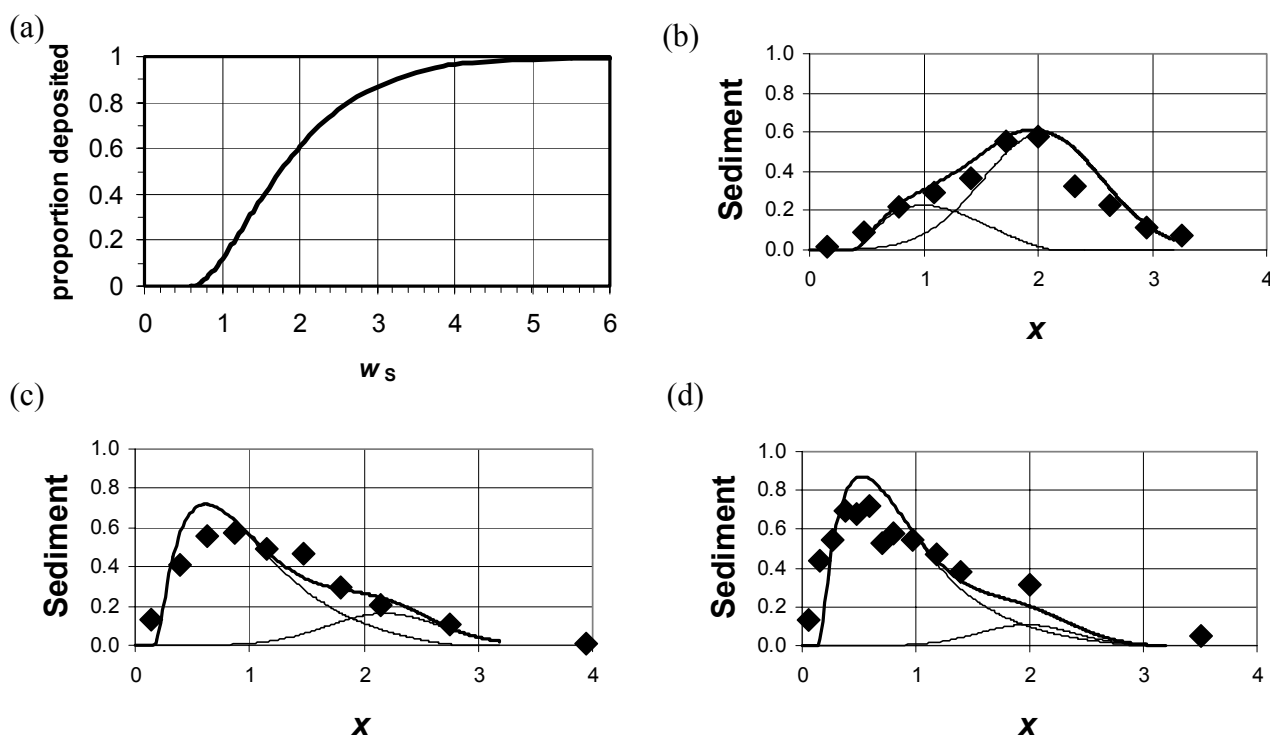
Figure 2 (a) Proportion of sediment dropping out in the near-source region as a function of the non-dimensional fall speed w_s for a horizontal source. (b-d) Theoretical predictions (for horizontal sources) for the sediment dropping out near the source and once the jet has reached the surface (thin lines for the two components, thick line for the sum) with symbols for the experimental measurements, with w_s = (b) 1.21, (c) 2.62 and (d) 3.13.
