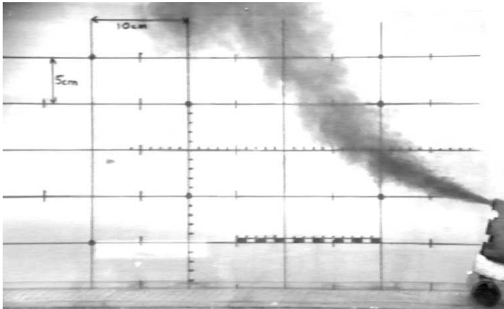
Figure 1. Angled turbulent buoyant jet (no particles), with the source angled slightly above the horizontal. The jet is dyed and the scale of the laboratory experiments is clearly marked. The free surface is just above the top of the picture and some of the spreading surface current can just be seen (especially towards the left).
