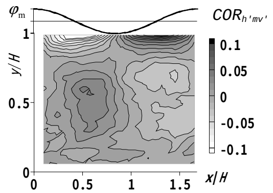
Figure 3 Spatial correlation coefficients of the surface fluctuation component of the eigenvector and the vertical component of the velocity fluctuations. The profile of the corresponding eigenvector is indicated above the contour map. POD mode m = 7 , Re_* = 505 , Fr = 1.23 .
