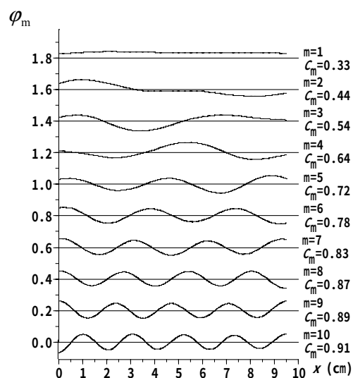
Figure 2 POD eigenvectors of the water surface fluctuations. The vertical axis is modified in 0.2 between two successive modes, m and m+1 . Re_* = 505 , Fr = 1.23 .
