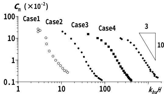
Figure 4 Streamwise spectrum of the water surface fluctuation. The values in horizontal axis are modified by multiplying 5, 5^2 , 5^3 in Case2, 3, 4, respectively. Fr = 0.54, 0.64, 0.85, 1.23 in Case1,2,3,4, respectively.
