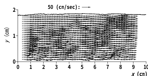
Figure 1 Instantaneous velocity vectors with the corresponding water surface profile ( Re_* = 505 , Fr = 1.23 ).
