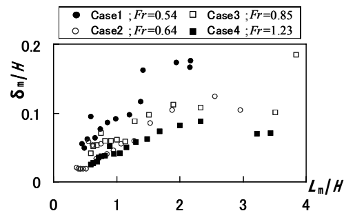
Figure 5 Relationship between the thickness of the surface influence layer and the wavelength of the surface fluctuation. Re_* = 505 , Fr = 0.54 - 1.23 .
