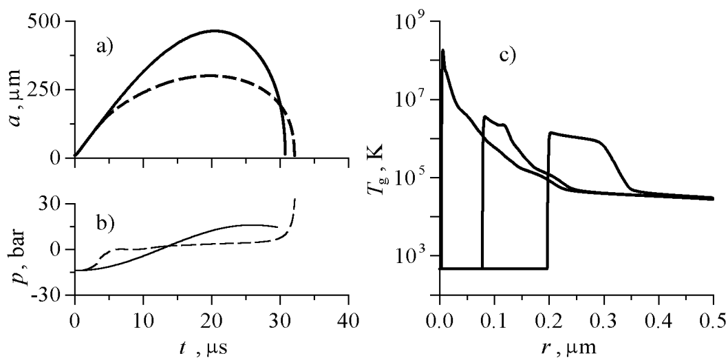
Figure 1. Bubble radius (a) and liquid pressure (b) evolution in time. Solid line – single bubble, dashed line – bubble in 20-bubbles cluster. Focusing of a shock wave near the bubble center (c).
