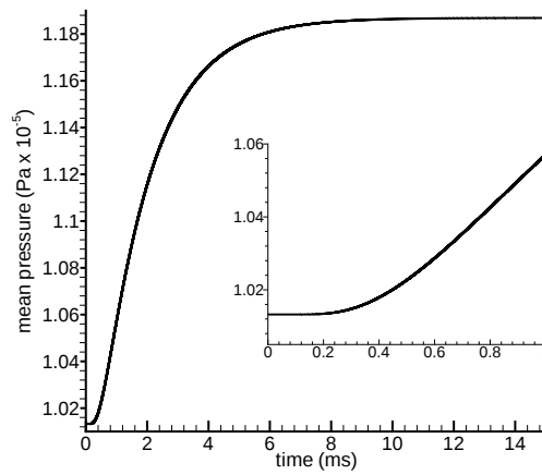
Figure 1. Case 2 : mean pressure vs. time
