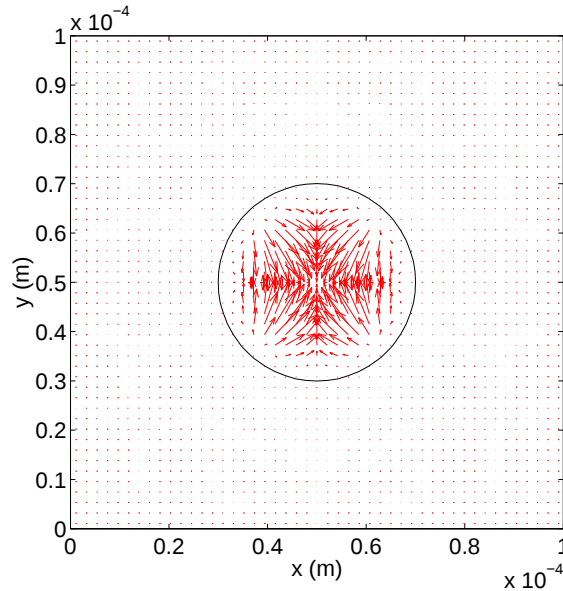
Figure 2. Case 2 : velocity field at t = 2,5ms
