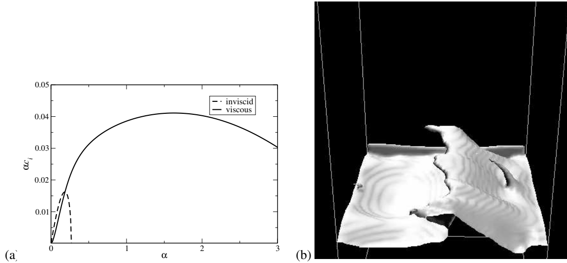
Figure 1. (a) Comparison of inviscid and viscous results, the parameters are We_g = 200 , Re_g = 1000 , \mu_g/\mu_l = 0.025 , \rho_g/\rho_l = 0.02 (b) 3D temporal growth of the instability. \rho_g/\rho_l = 0.1 , We_g = 200 , Re_g = 1000 , the grid size is 128^3 .
