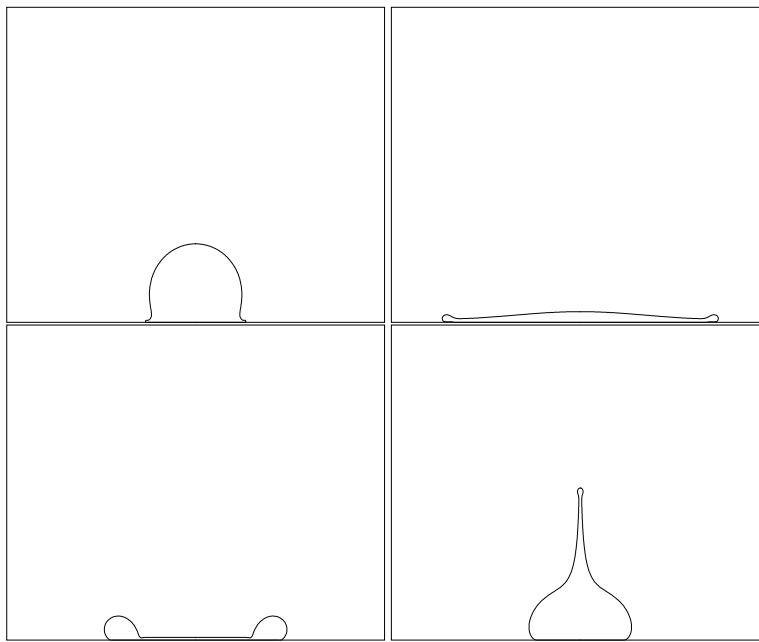
Figure 1. Drop shapes during the impact of a 3 mm water drop ( We = 540 and Re = 900 ).
